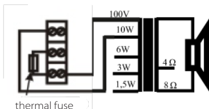
10W transformer connection diagram
