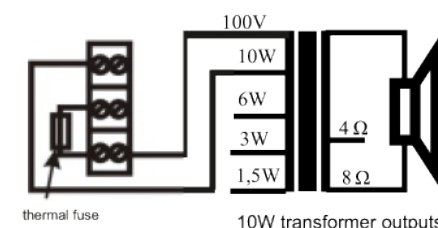
Scheme with the 10W transformer connections
