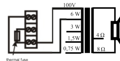
Scheme with the 6W transformer connections
